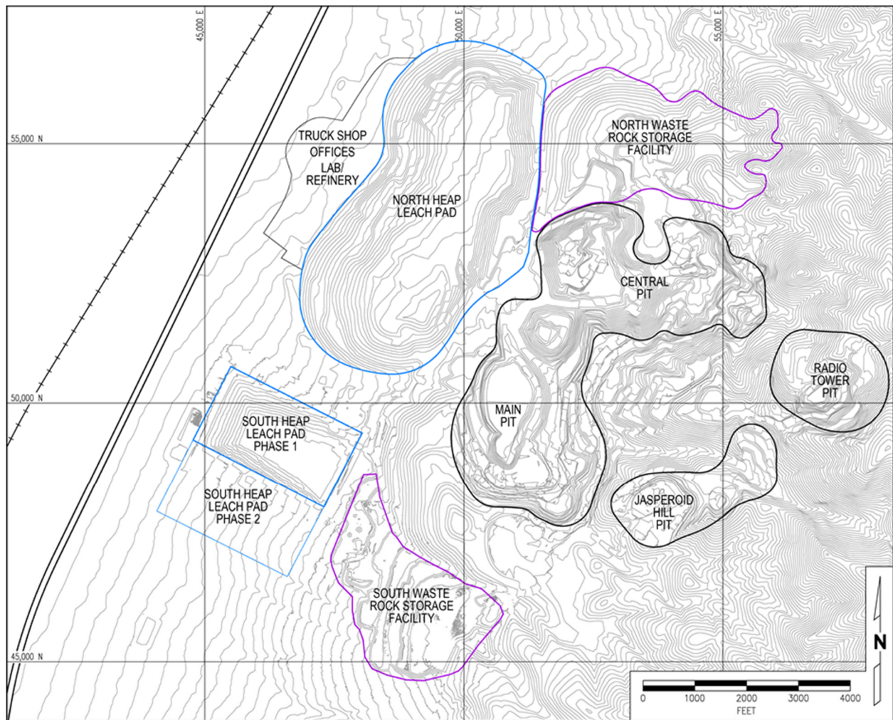
Figure 18-1 Site General Arrangement, Source IMC 2020
