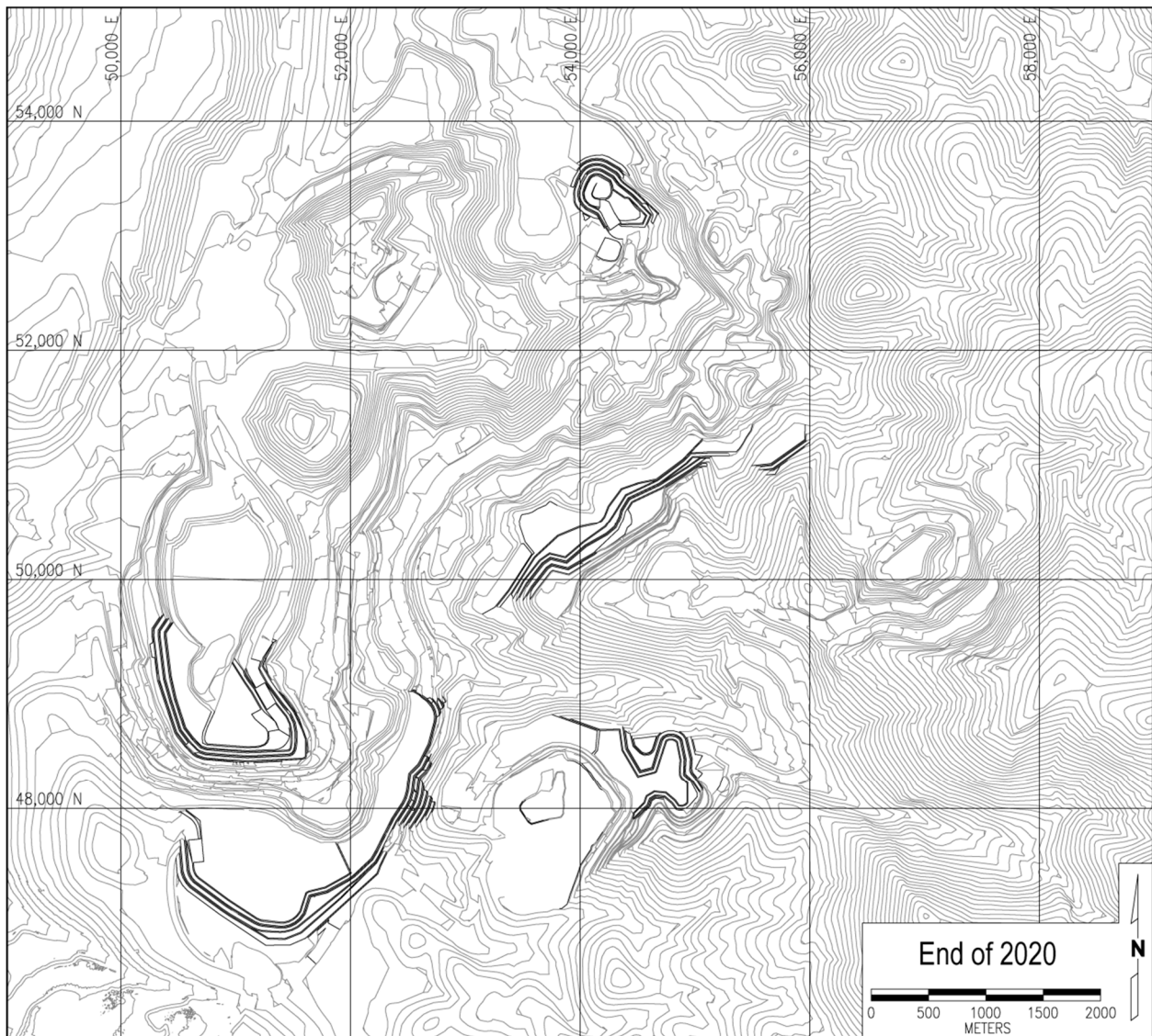
Figure 16-2 Annual Mine Plan Illustrations, end of Year 2020
