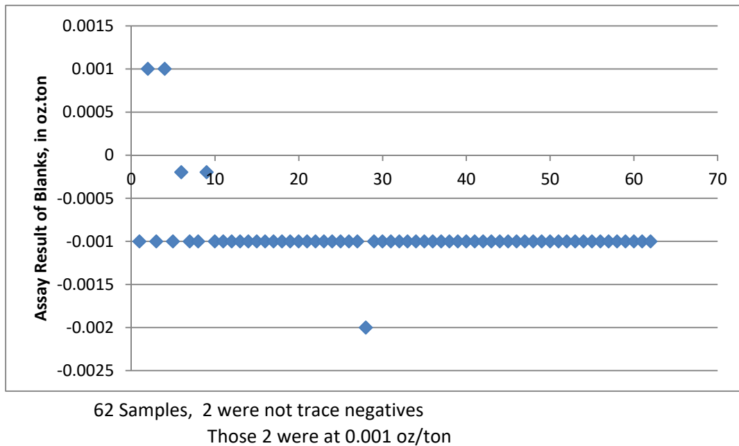
Figure 12-2 AAL Internal Lab Blanks, 2017 Drill Program
