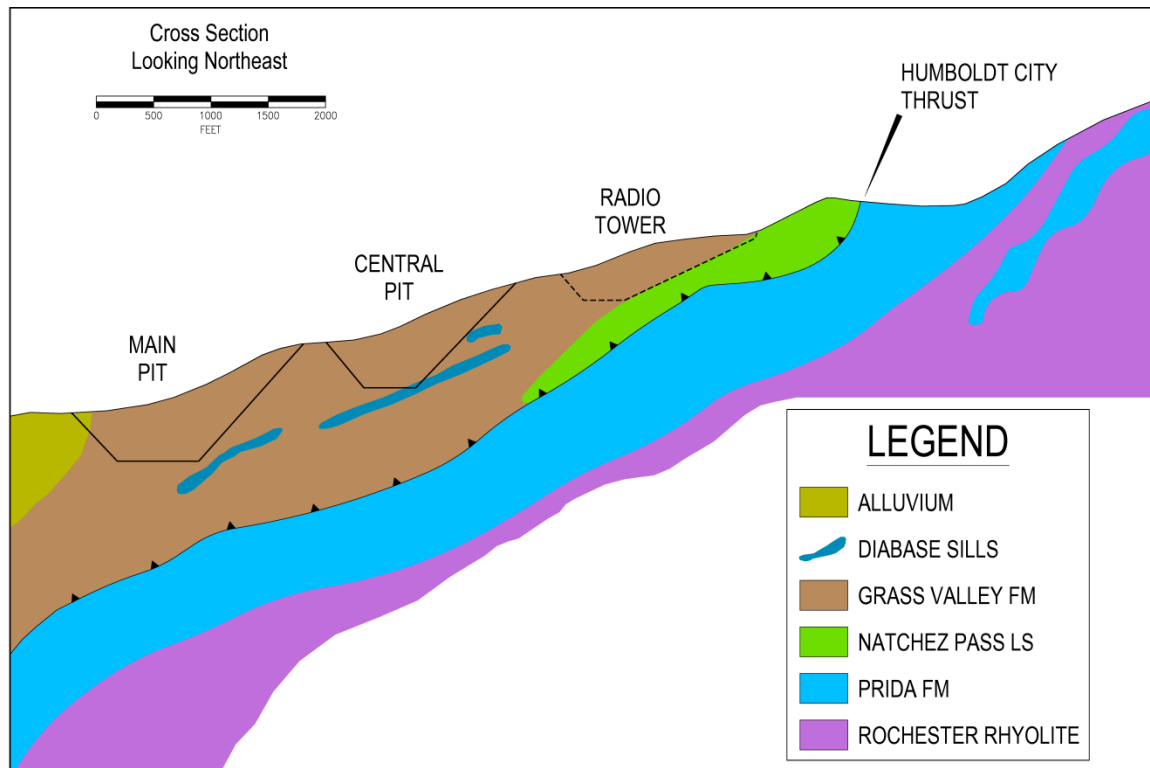
Figure 7-2: Florida Canyon Generalized Geologic Cross Section
