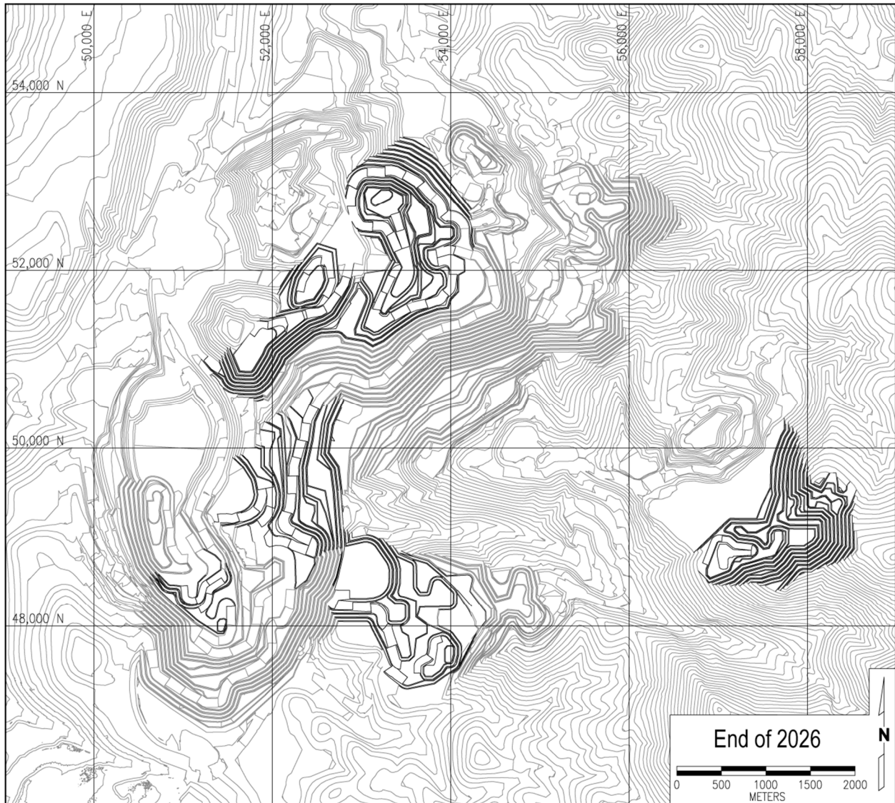
Figure 16-4 Annual Mine Plan Illustrations, end of Year 2026
