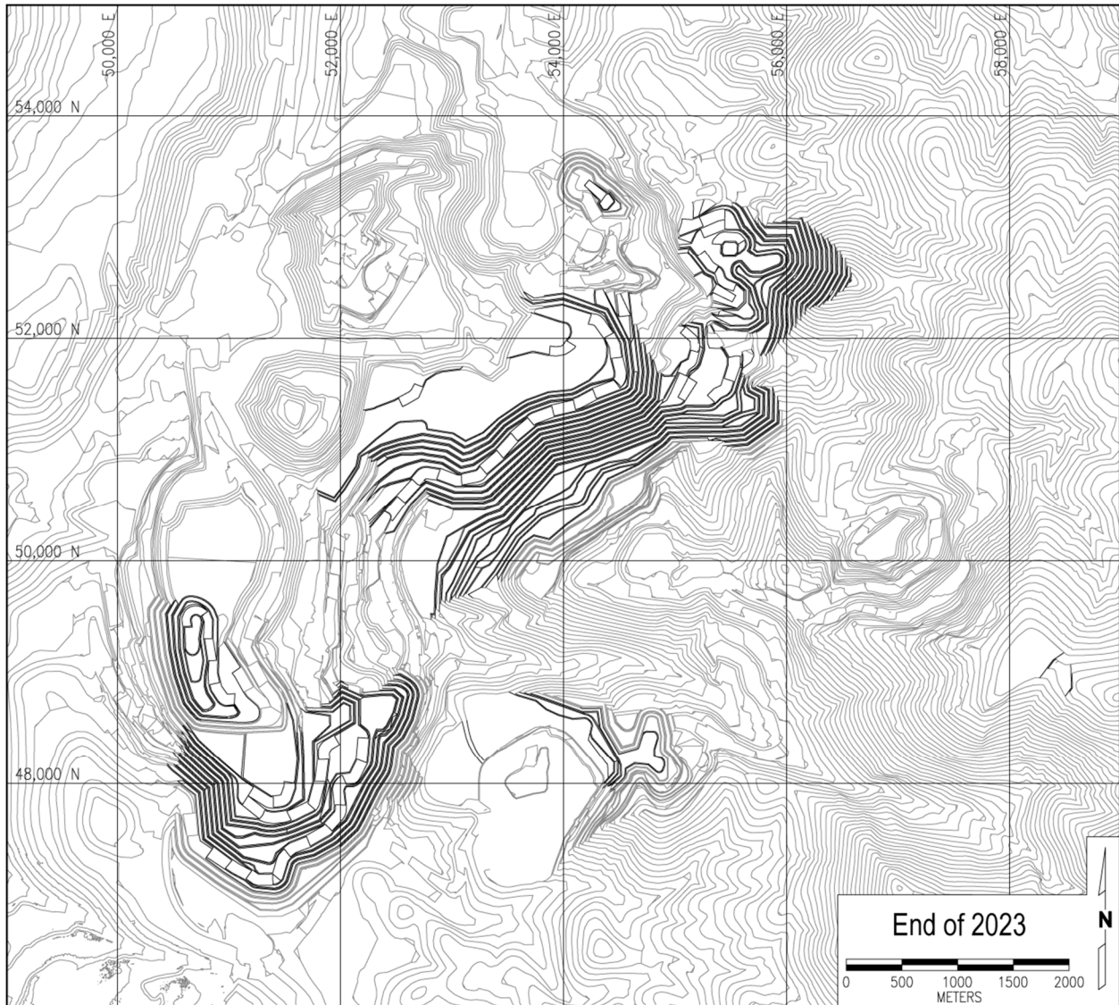
Figure 16-3 Annual Mine Plan Illustrations, end of Year 2023
