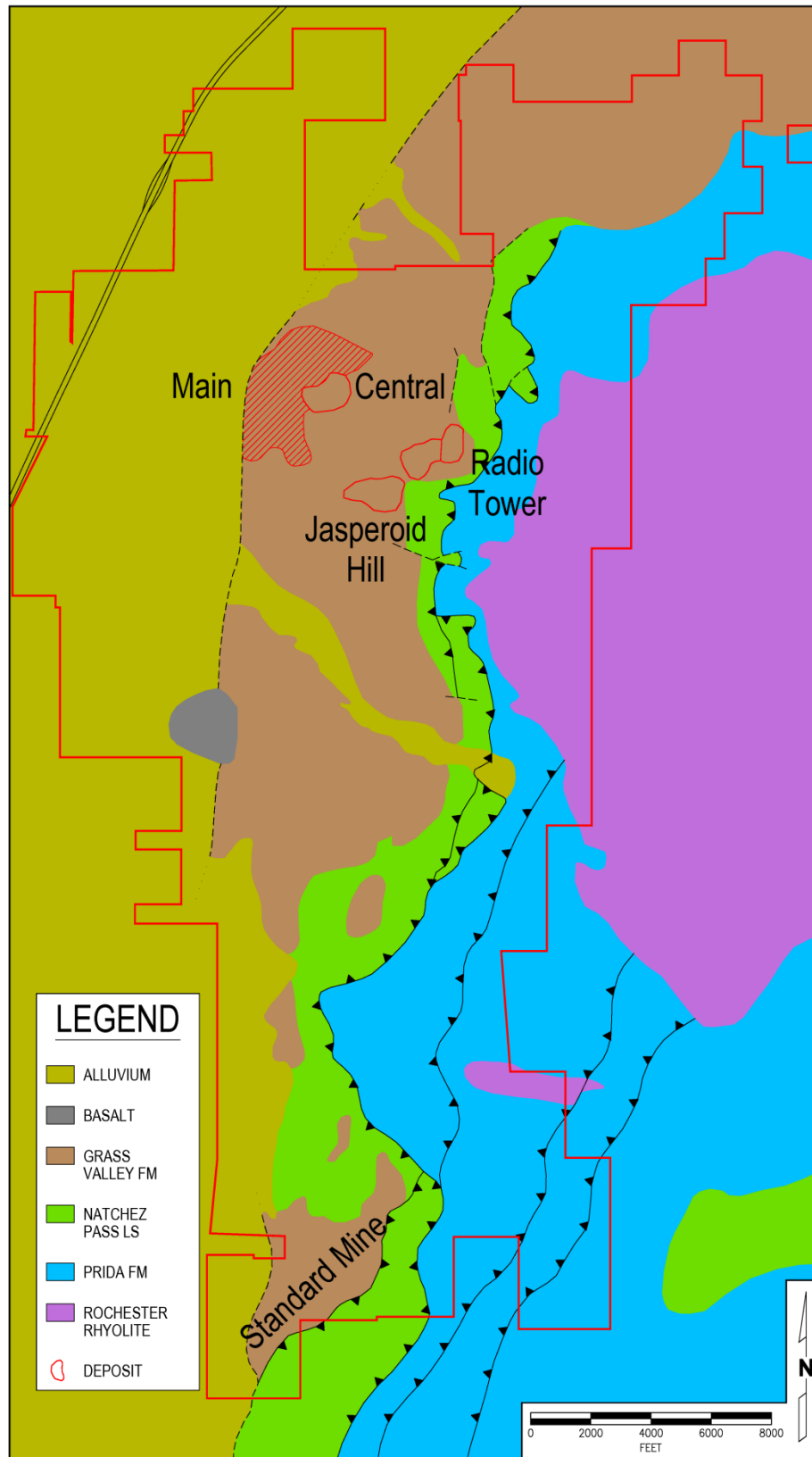
Figure 7-1: Florida Canyon Area Geology
