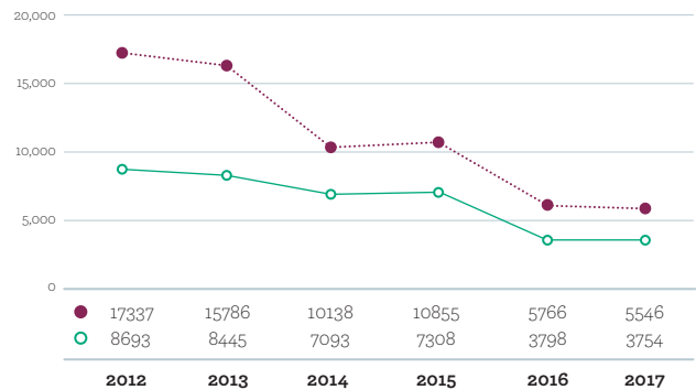
SO2 EMISSIONS (TONS)
