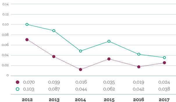
PM10 EMISSION RATE (LB/MWH)
