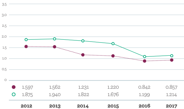
NOX EMISSION RATE (LB/MWH)
