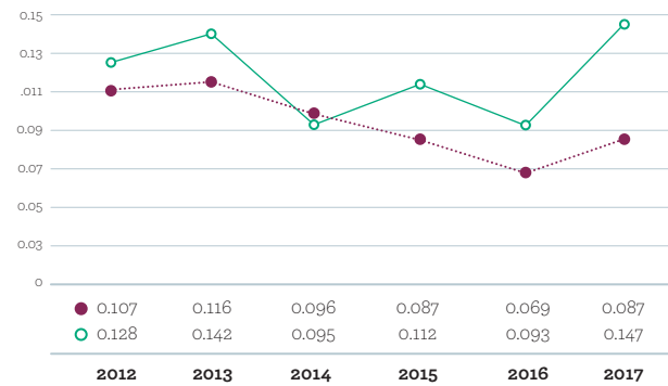
CO EMISSION RATE (LB/MWH)
