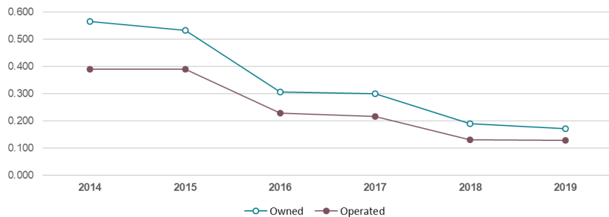
SO2 EMISSION RATE (LB/MWH)
